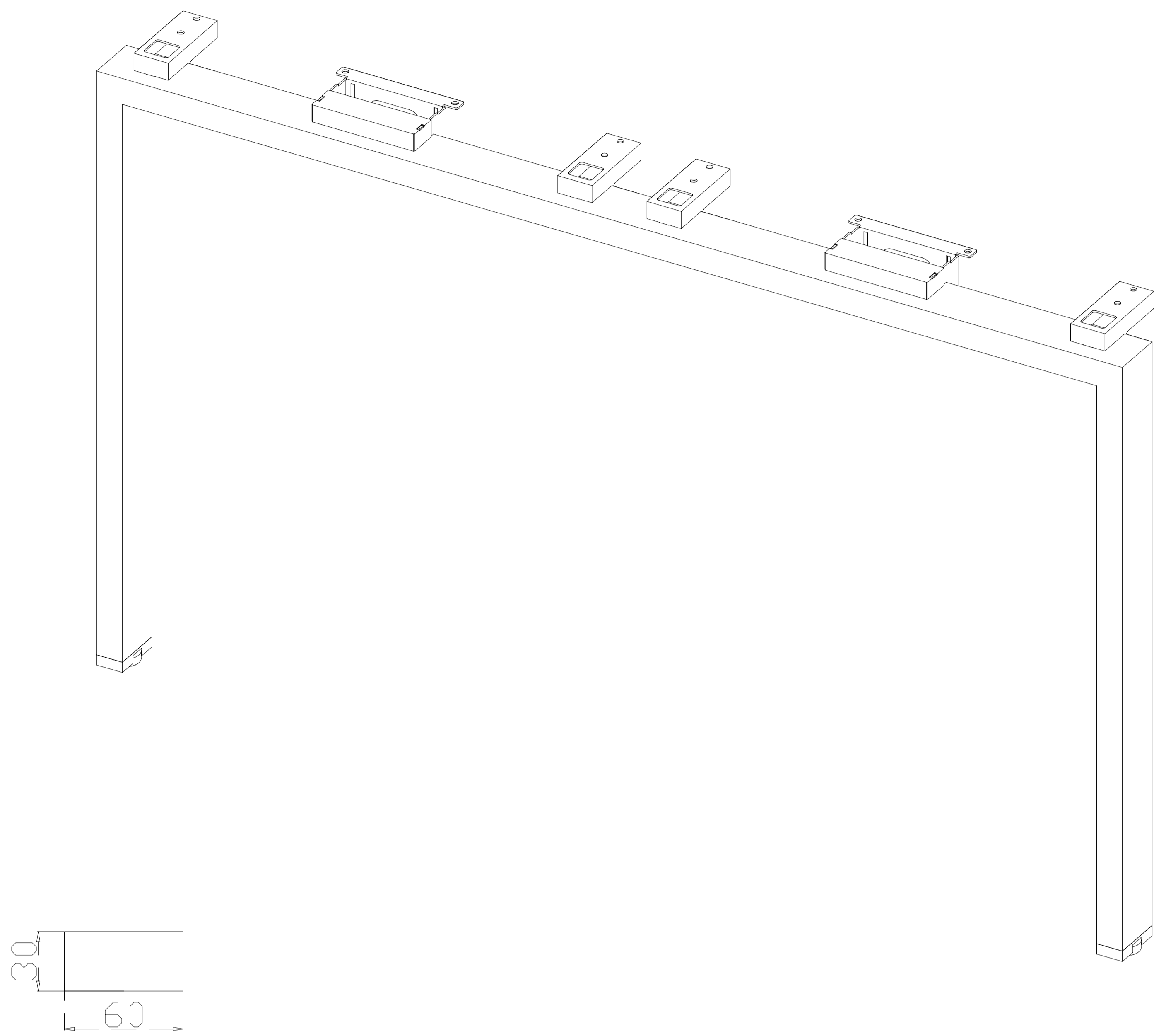
Q 7612 * 1200 mm
